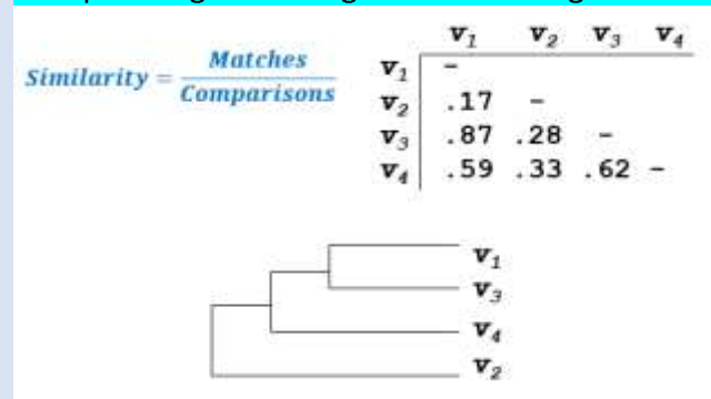
Figure 0.20 Similarity Matrix
