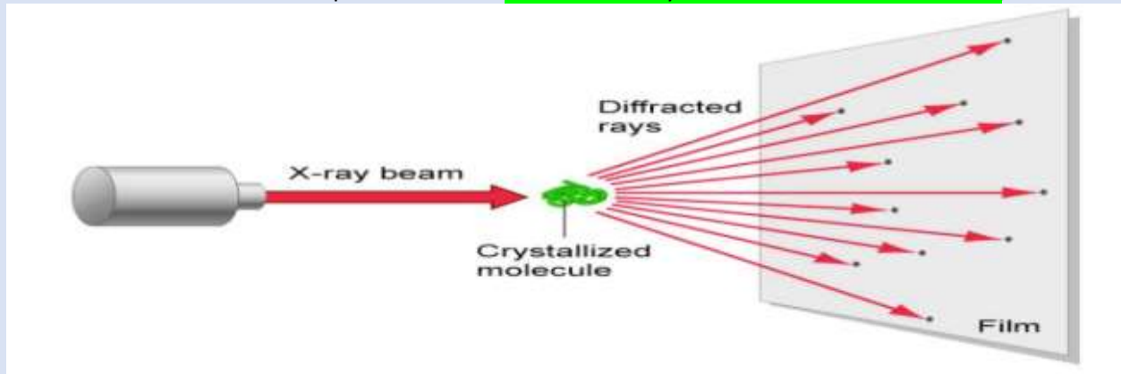
Figure 13 X-ray Crystallography
