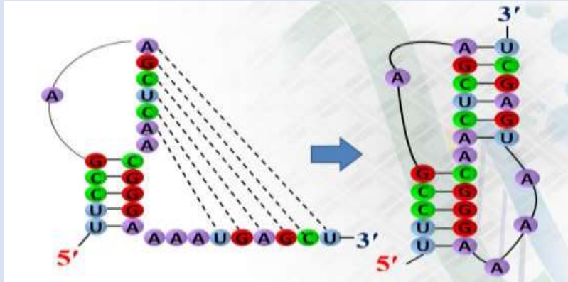
Figure 12 pseudoknots
